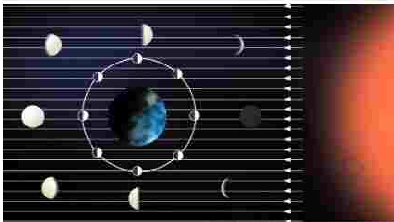
Fig. 17.5: Positions of the moon in its orbit and its corresponding phases
